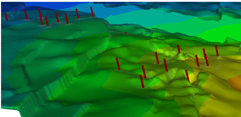
Visualisation of reservoir temperature in a 3D FEFLOW model.
