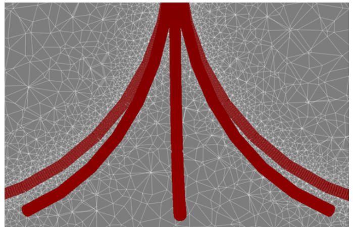
Modelling of deep inclined geothermal wells.
