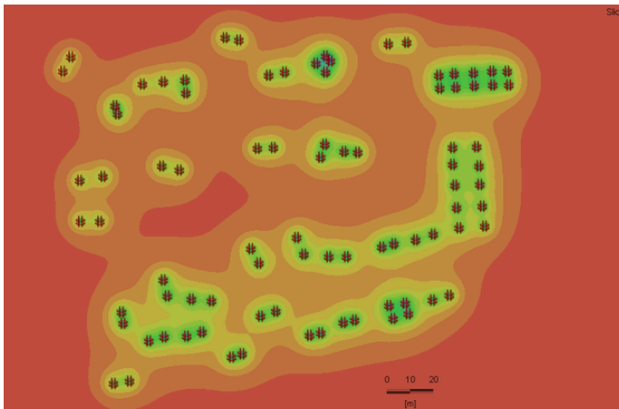
Temperature distribution around multiple Borehole heat exchangers.
