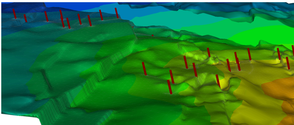
Visualisation of reservoir temperature in a 3D FEFLOW model.
